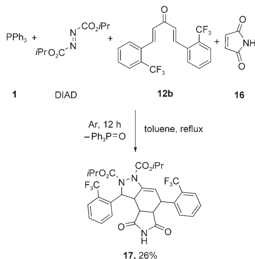
Scheme 8. Synthesis of an indazole derivative.
